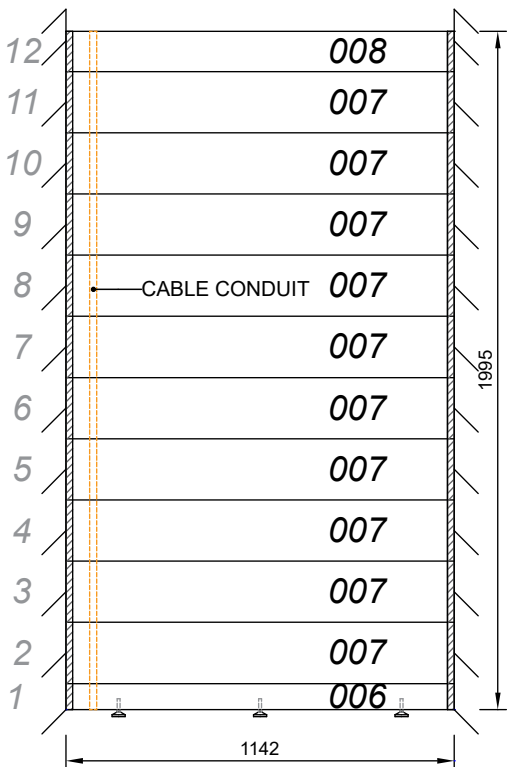
WALL B (BACK) VIEW FROM THE INSIDE
