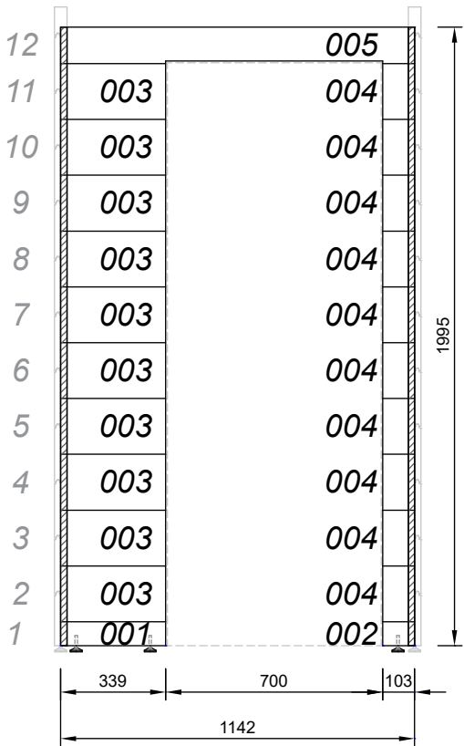
WALL D (FRONT) VIEW FROM THE OUTSIDE
