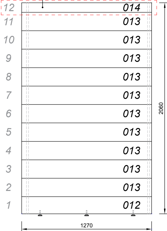
WALL C (RIGHT) VIEW FROM THE OUTSIDE
