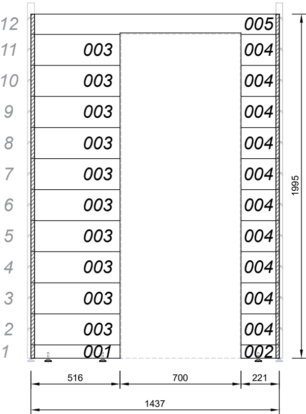
WALL D (FRONT) VIEW FROM THE OUTSIDE
