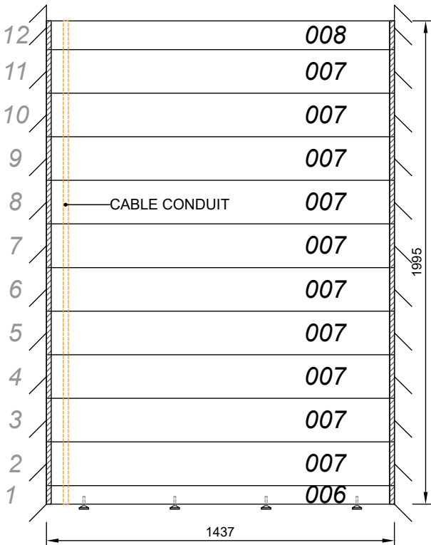
WALL B (BACK) VIEW FROM THE INSIDE
